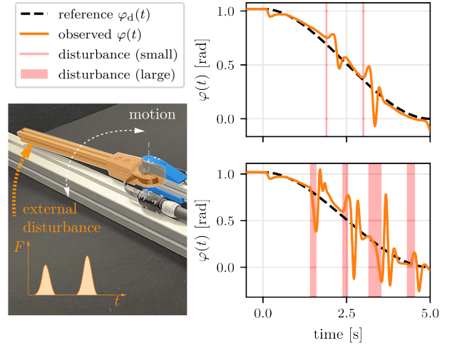
Fig. 6. Tracking performance of ANODEC in two disturbed trials. In the first trial (top) there are two small disturbances (poking the endeffector with a stick) whereas in the second trial (bottom) there are four large disturbances (grabbing and briefly holding the endeffector). ANODEC remains stable and behaves as expected in both trials.
