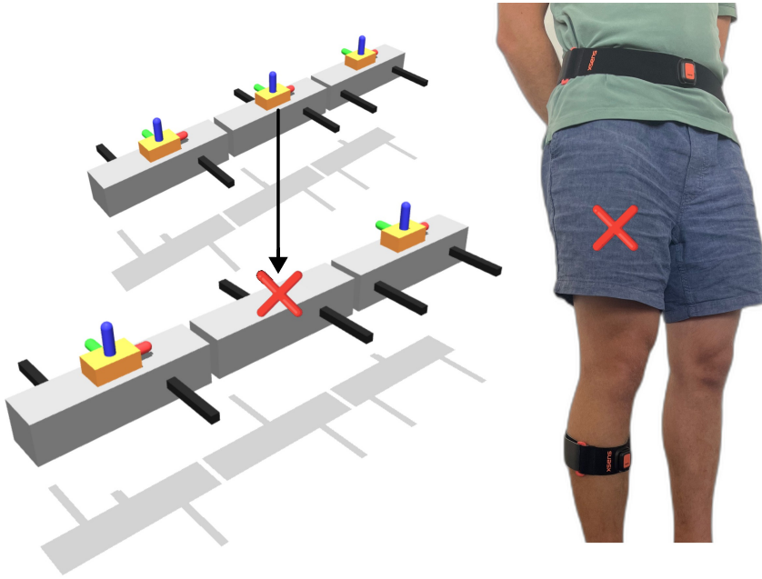
Figure 2.6: Sparse IMT uses less than one sensor per segment. A three-segment with no IMU on the middle segment; a model of a human leg that consists of the KC of hip, thigh, and shank.
