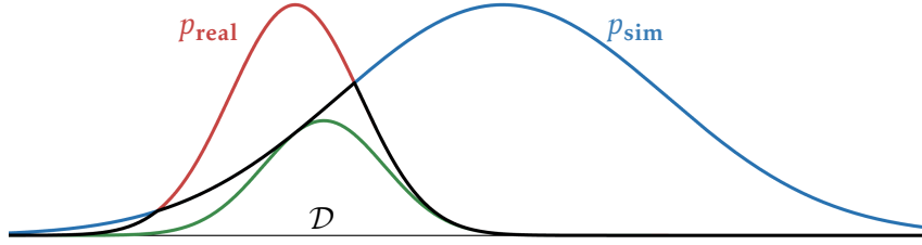
Figure 2.2: Sim-to-real transfer requires that the simulated training data distribution p_{sim} ideally maximizes the overlap (black) or joint distribution (green) of simulated (blue) and real-world (red) data.
