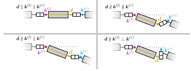
Fig. 4. Four different double-hinge-joint systems corresponding to different realizations of the joint axes directions.
