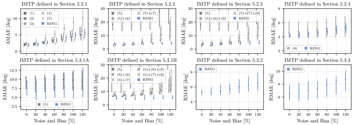
Figure 9: Comparison of the robustness of RING and SOTA methods as the level of noise and bias is increased. To simulate reasonable noise and bias offset ranges, we constructed a worst-case IMU by combining the worst properties of various IMU manufacturers, as summarized in Table 3. Then, those worst-case noise and bias values are incrementally (in seven equidistant steps) increased from 0 to 120%, and a corresponding amount of simulated noise and bias is added to our real-world IMU data (see Section 5.1), which yields seven modified datasets. RING and all SOTA methods are validated on the modified dataset, and this procedure is repeated using ten different seeds. The AMAEs and RMAEs of all methods are plotted for all IMTPs as a function of the seven steps. The 25%/50%/75%-percentiles across all trials and seeds are shown, and they show that RING maintains accuracy comparable to SOTA methods in all IMTPs and, especially in two-segment KC tracking, substantially outperforms them. Methods are Weber et al. (2021)(1), Madgwick (2010)(2), Mahony et al. (2008)(3), Seel & Ruppert (2017)(4), Laidig & Seel (2023)(5), Laidig et al. (2017)(6), Lehmann et al. (2020)(7), Olsson et al. (2020)(8), Bachhuber et al. (2023)(9).
