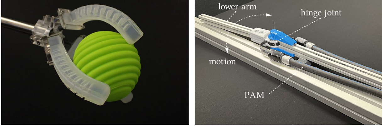
Figure 2.7: A SR that grips a ball (left side; image reused with explicit consent 4 ) and a robot arm actuated by a PAM (Pneumatic Artificial Muscle) (right side; adapted from Bachhuber et al. (2024a)). Both systems are complex and difficult to model, making data-driven control methods desirable.
