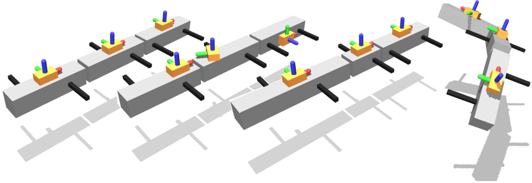
Figure 2.3: Domain randomization techniques for a three-segment (grey boxes) KC (Kinematic Chain) with body-attached IMUs (orange boxes). The second KC is obtained by randomizing the IMUs attachment. Similarly, the third KC is obtained by randomizing the length of the segments, and the initial pose is randomized in the last KC. An RNN can be trained to estimate the rotational state of the KC from the IMU measurements by simulating random motion and the corresponding virtual IMU measurements. Suitable domain randomization techniques enable the trained RNN to generalize from simulation to experiment.
