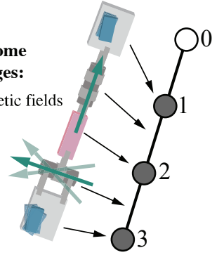
Fig. 1. A three-segment KC with two IMUs (blue boxes). The graph representation of the KC is given by the parent array \lambda = (0, 1, 2)^T . The neural network-based multiple-IMU sensor fusion algorithm RING receives the graph representation and IMU data as input and estimates the rotational state of the KC, overcoming all four key challenges of IMT simultaneously.
