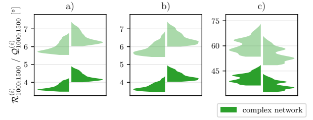
Fig. 8. Estimated distribution of the RMSE \mathcal{R}_{1000:1500}^{(i)} and 90-percentile \mathcal{Q}_{1000:1500}^{(i)} of inter-segment orientations i (left/right split) as estimated by the RNN-based observer for three different three-segment kinematic chains: a) biaxial joint and hinge joint with linearly dependent joint axes; b) biaxial joint and hinge joint with linearly independent joint axes; c) two triaxial joints, i.e. no restrictions on relative motions.
