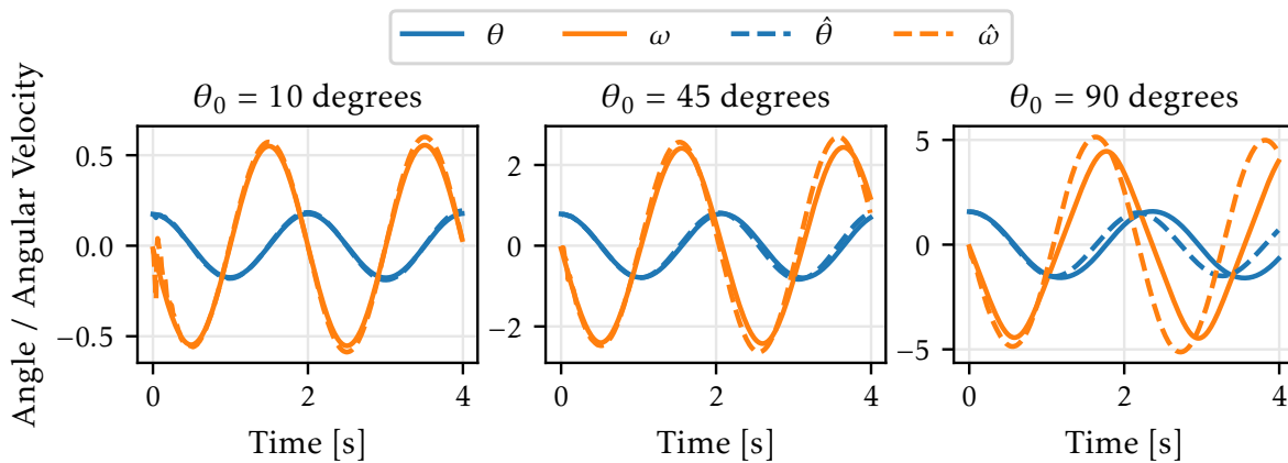
Figure 1.4: A Kalman filter is used to track the state ( \theta and \omega , and \hat{\theta} and \hat{\omega} is the state estimate) of a pendulum from its Cartesian x-position. As the initial pendulum angle \theta_0 increases, the linearization of the nonlinear dynamics breaks down, and the tracking accuracy of the observer decreases.
