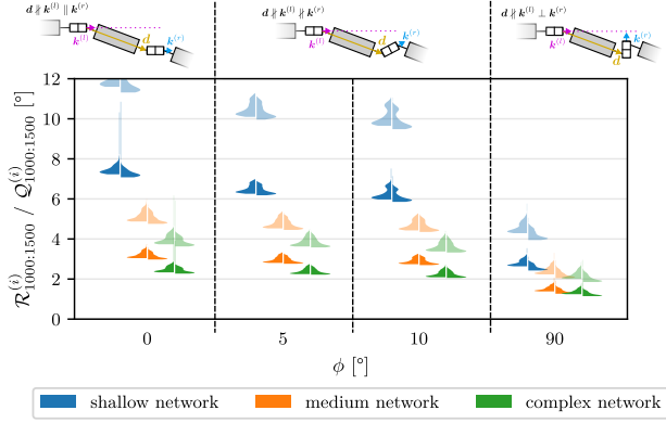
Fig. 7. Estimated distribution of the RMSE \mathcal{R}_{1000:1500}^{(i)} and 90-percentile \mathcal{Q}_{1000:1500}^{(i)} of inter-segment orientations i (left/right split) as estimated by the RNN-based observer. For each of the three network complexities, the residual error increases as \phi decreases, i.e. as the two joint axes of the double-hinge-joint system align.
